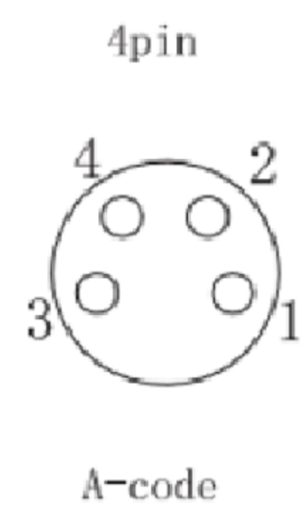
Pin assignment front view/针位分布前视图
